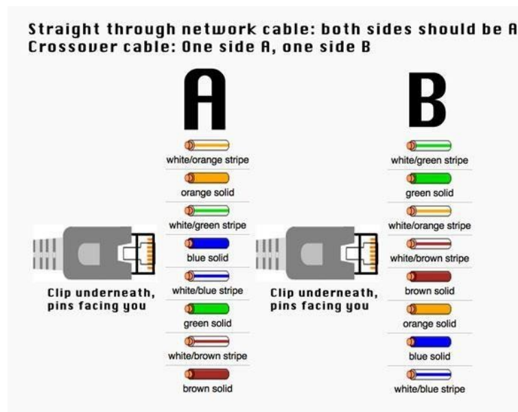
Fig. 2 — T568A / T568B wire colour arrangement used at each end
